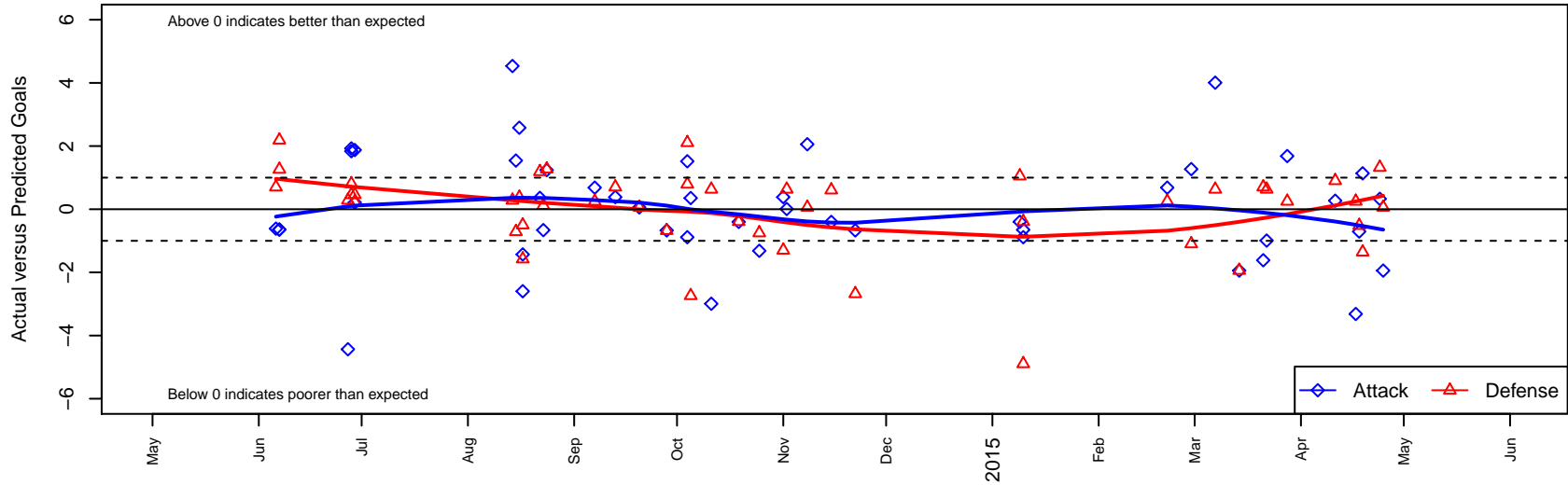
Normandy Park SC Blue G03 Dots are actual minus expected GF (blue circles) and GA (red triangles). Blue line is smoothed change in attack strength. Red is smoothed change in defense strength.
